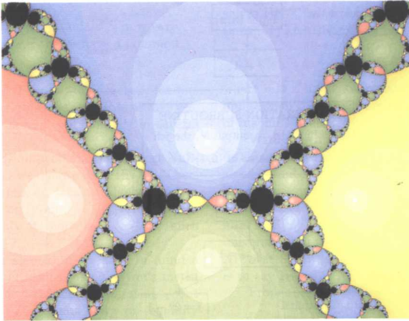
Fig. 9. The dynamics of the Newton endomorphism for f(z) = (z^2 - 1)(z^2 + 0.16) . Courtesy of S. Sutherland and Springer-Verlag.
