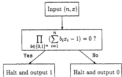
Fig. 11. An algebraic machine for solving the Knapsack problem.
