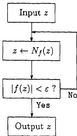
Fig. 8. The Newton machine for f .
