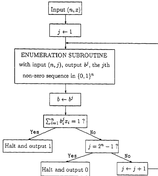
Fig. 10. Exhaustive search machine for solving the Knapsack problem.
