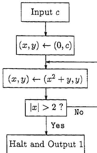
Fig. 3. A flow chart associated with the Mandelbrot set.
