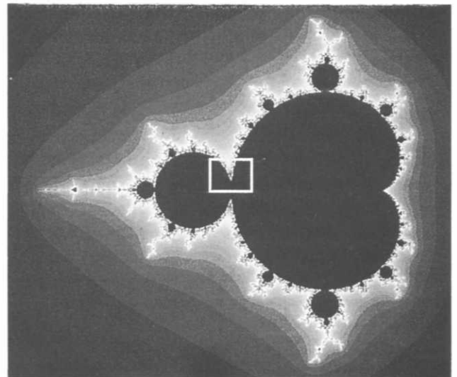
Fig. 1. The Mandelbrot set. (Courtesy of H.-O. Peitgen and Springer-Verlag.)
