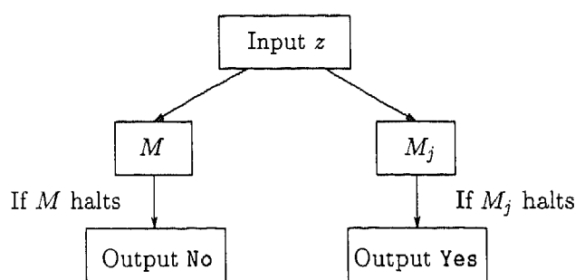
Fig. 7. J is decidable (supposing J is a halting set).
