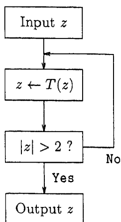
Fig. 5. A Julia set flow chart.
